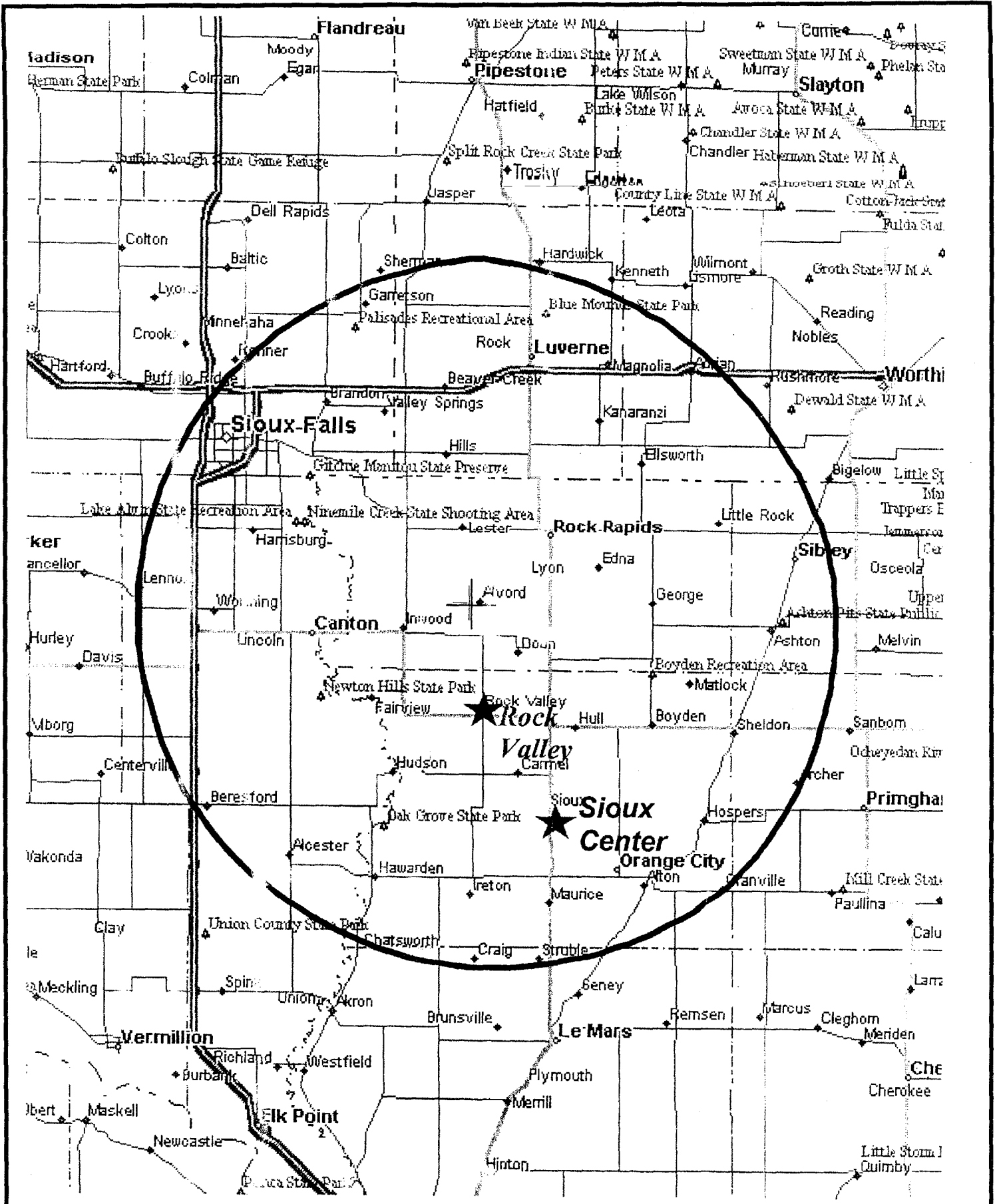
KIHK .5 mV/m coverage Based on FCC 50/50 coverage charts
